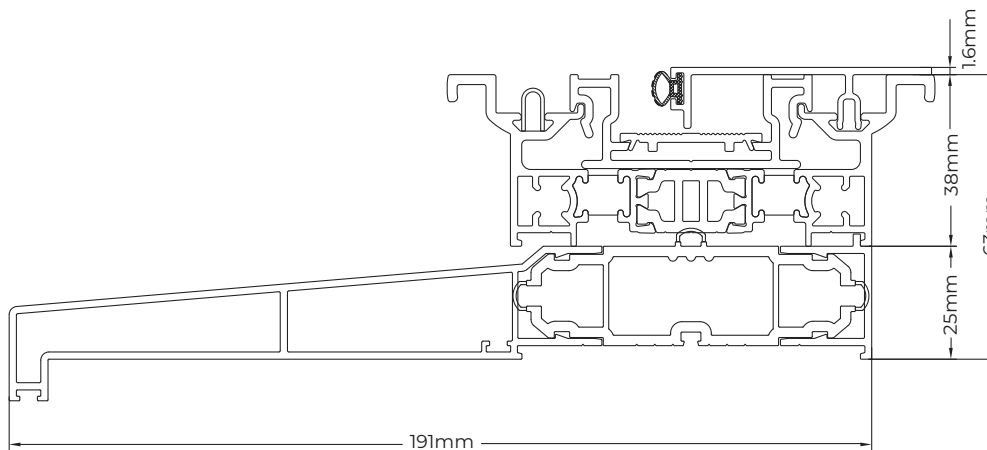
Standard outerframe with large cill
