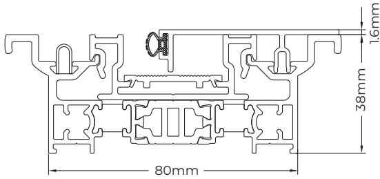
Standard Outerframe
