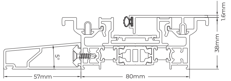
Standard outerframe with large cill
