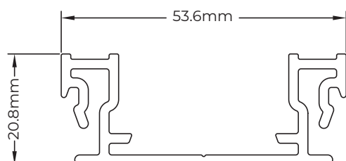
SGP510 OUTER FRAME INSERT
