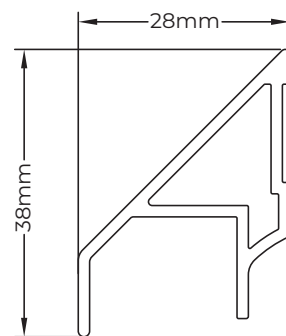
SGP013 HEAD DRIP
