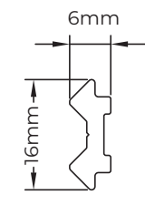
SA572 CILL NOSE BASE
