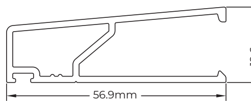
SA571 CILL NOSE
