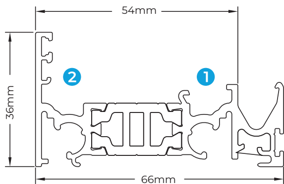
SGP501 HOOKED BEAD INTERLOCK
