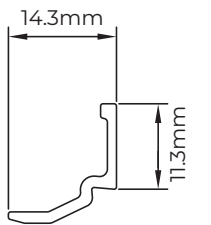
SGP404 40mm BEAD
