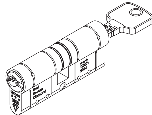
SGP606 - 3* 35/35 CYLINDER - to suit SGP611 SGP607 - 3* 40/40 CYLINDER - to suit SGP610
