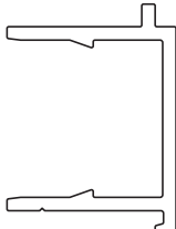
SA015 INTERNAL CILL TRIM / 25mm EXTENSION TRIM
