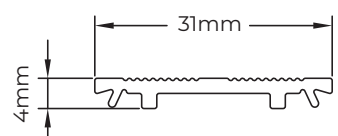
SA510 LOW THRESHOLD COVER STRIP
