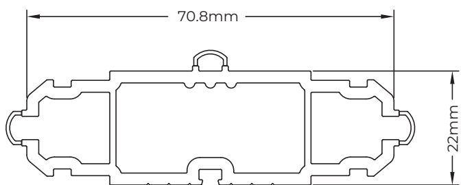
SA505 80mm ACCESSORY THERMAL BREAK
