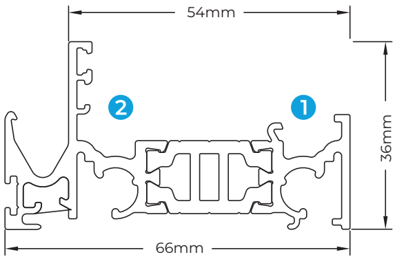
SGP500 HOOKED REBATE INTERLOCK
