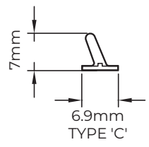
SG809 INTERLOCK GASKET
