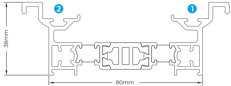
SGP100 OUTER FRAME
