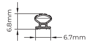
SG808 SLIDING GASKET
