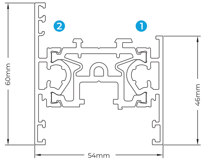
SGP301 CONTEMPORARY SASH
