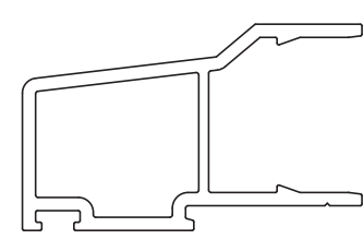
SA010 STUB CILL NOSE
