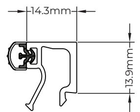
SGP400 28mm BEAD
