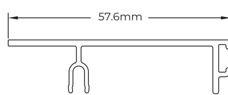
SGP010 FRAME TRIM
