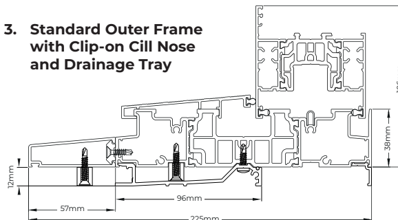
4. Standard 3-Pane Outer Frame with Drainage Tray
