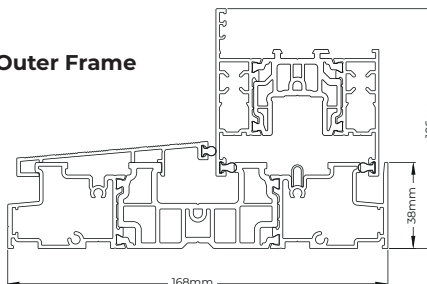
3. Standard Outer Frame with Clip-on Cill Nose and Drainage Tray
